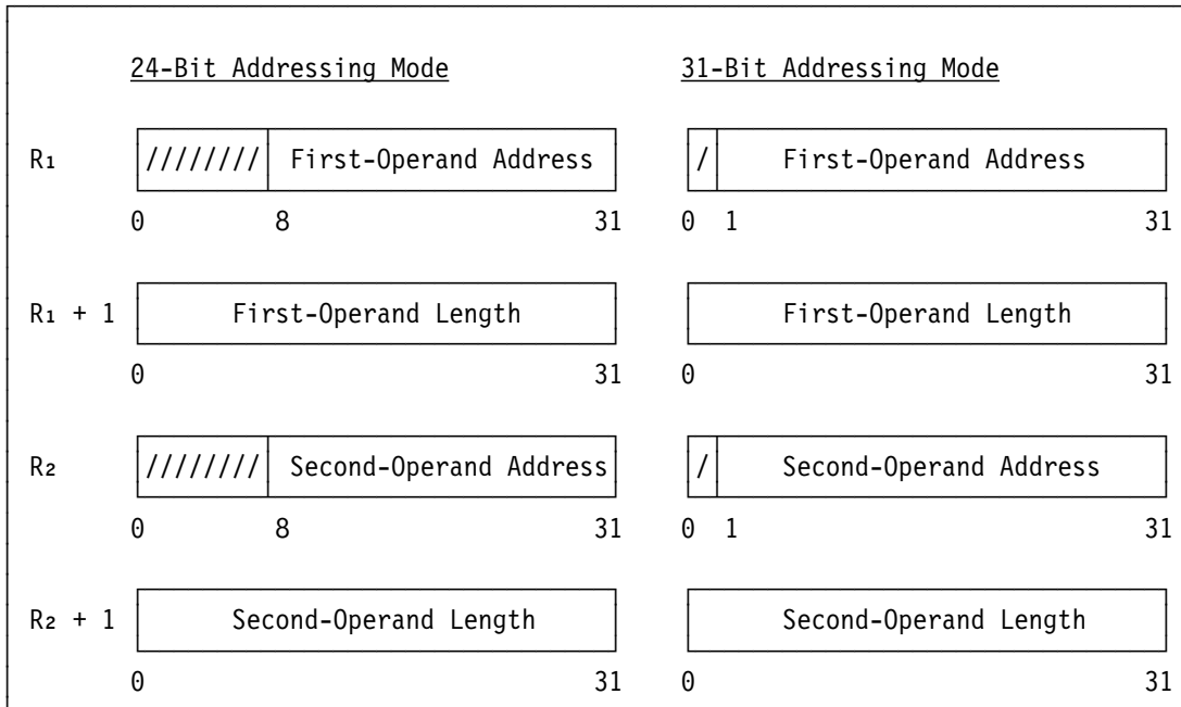
Figure 7-9. Register Contents for CONVERT UNICODE TO UTF-8
