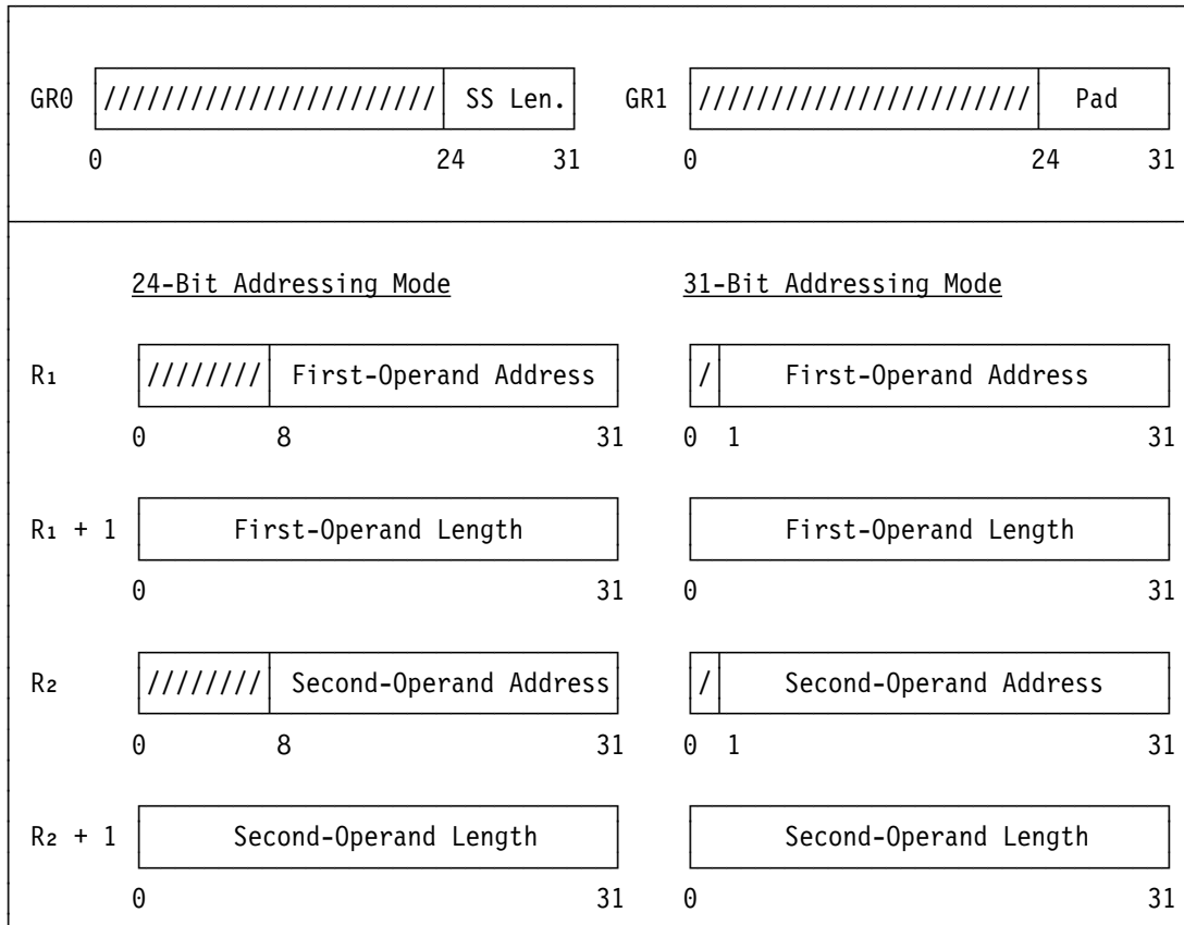
Figure 7-8. Register Contents for COMPARE UNTIL SUBSTRING EQUAL
