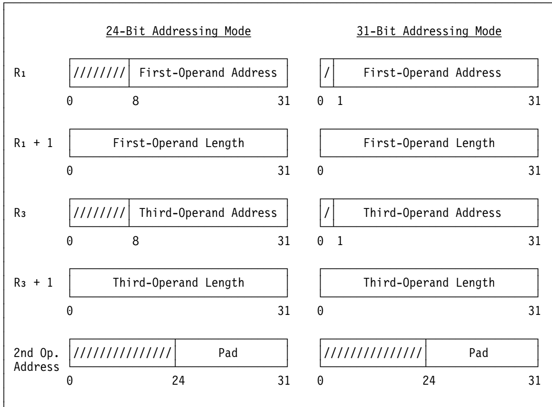
Figure 7-7. Register Contents and Second-Operand Address for COMPARE LOGICAL LONG UNICODE
