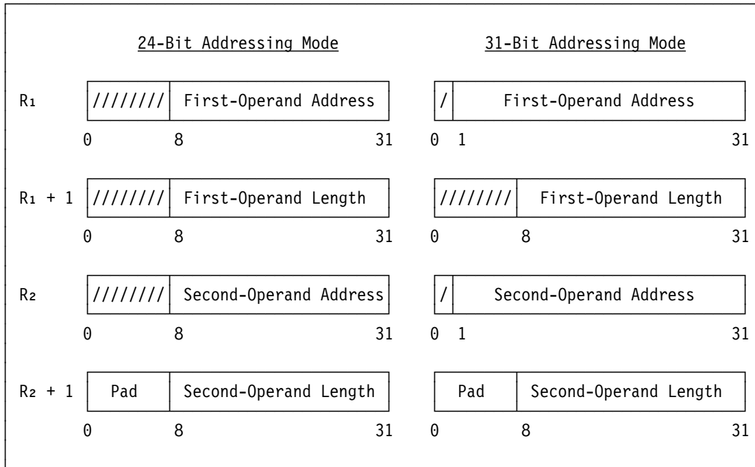
Figure 7-11. Register Contents for MOVE LONG
