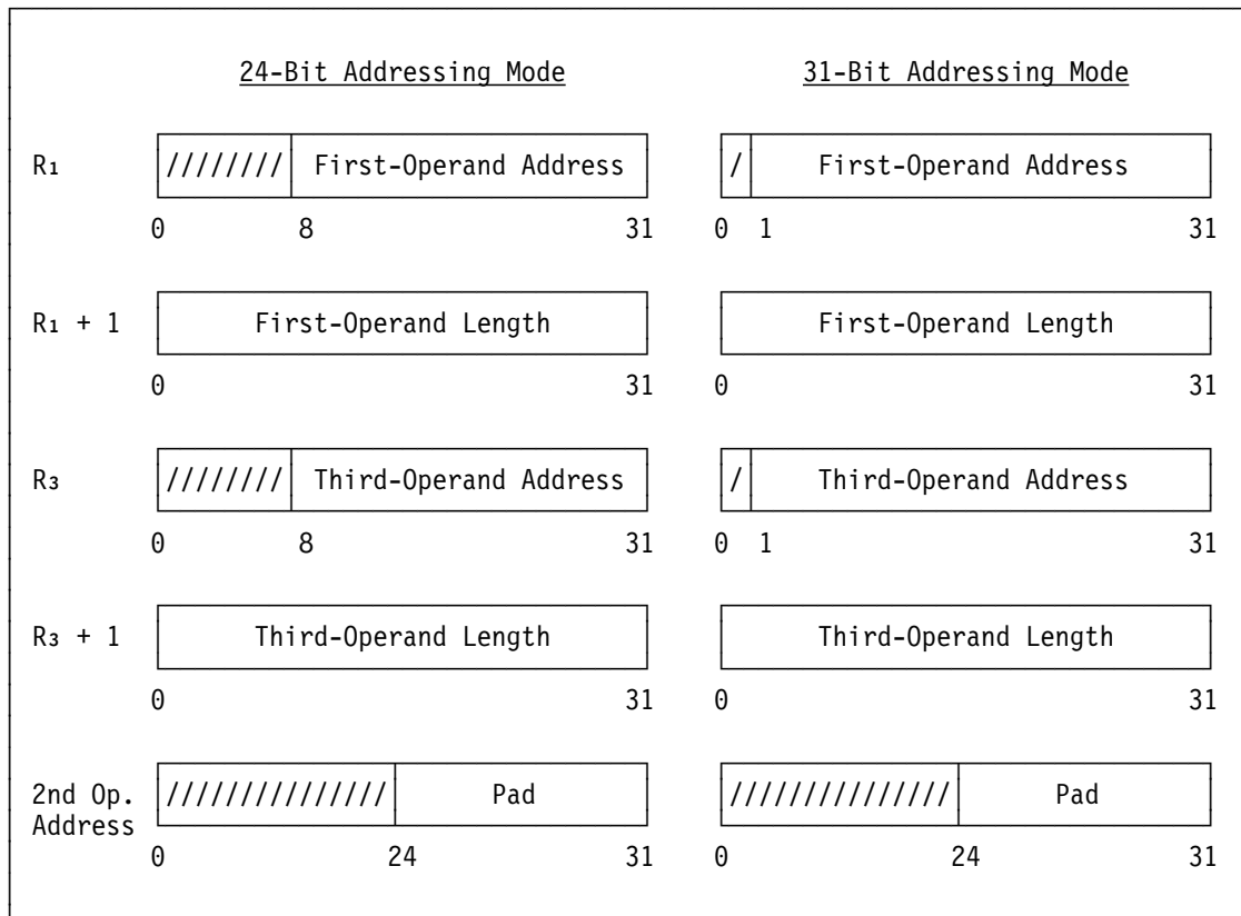
Figure 7-13. Register Contents and Second-Operand Address for MOVE LONG UNICODE
