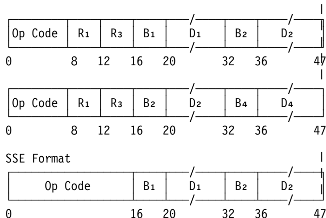
Figure 5-1 (Part 3 of 3). Basic Instruction Formats
