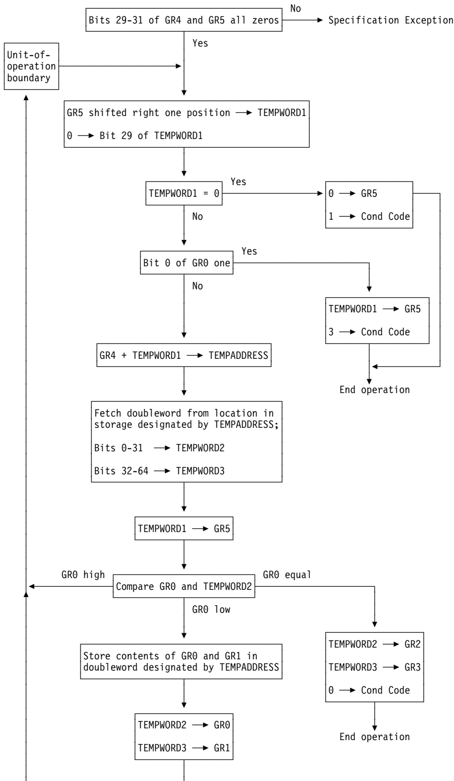
Figure 7-21. Execution of UPDATE TREE
