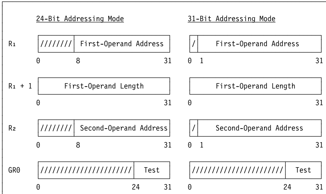
Figure 7-19. Register Contents for TRANSLATE EXTENDED
