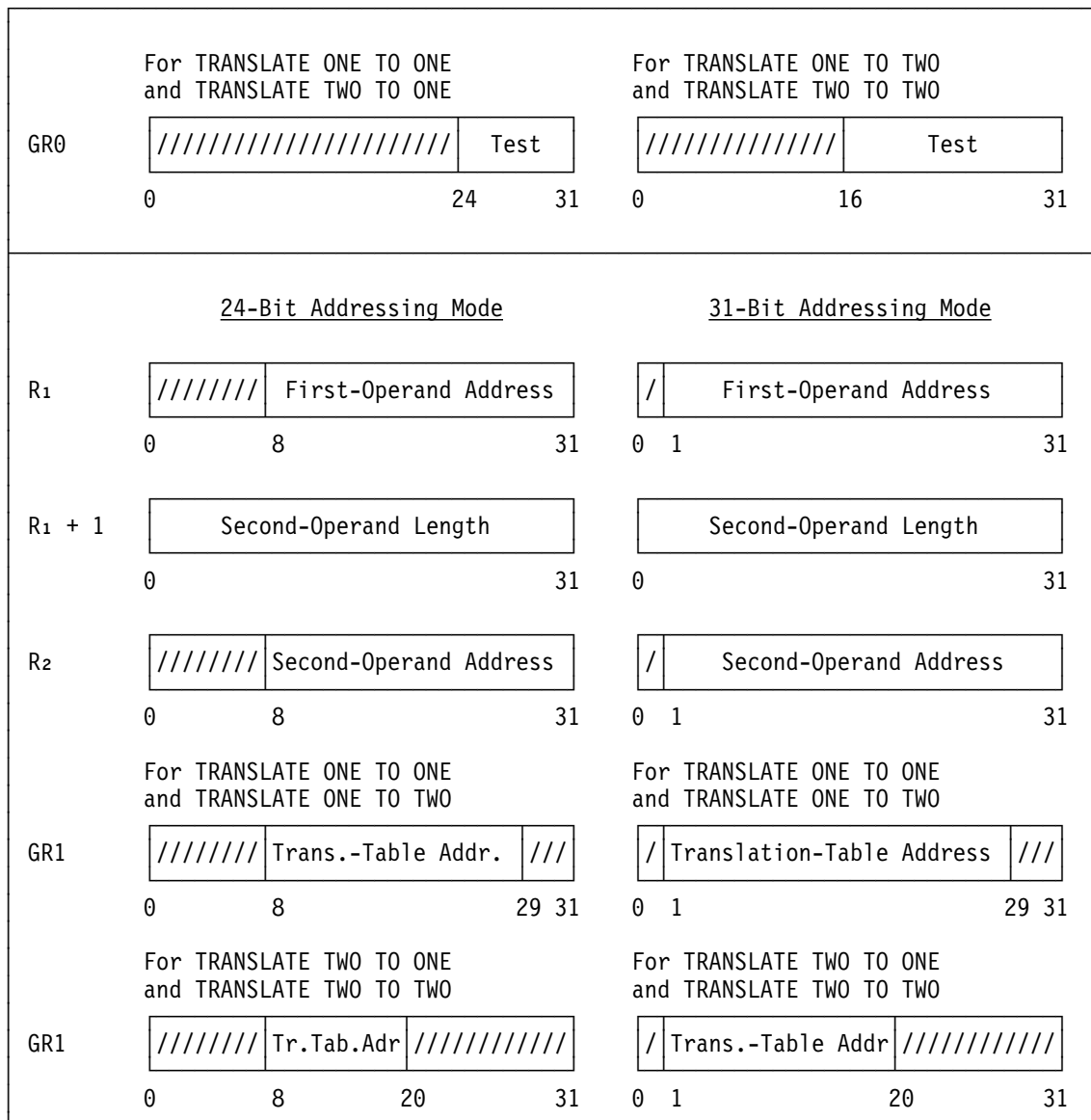
Figure 7-20. Register Contents for TRANSLATE ONE TO ONE, TRANSLATE ONE TO TWO, TRANSLATE TWO TO ONE, and TRANSLATE TWO TO TWO
