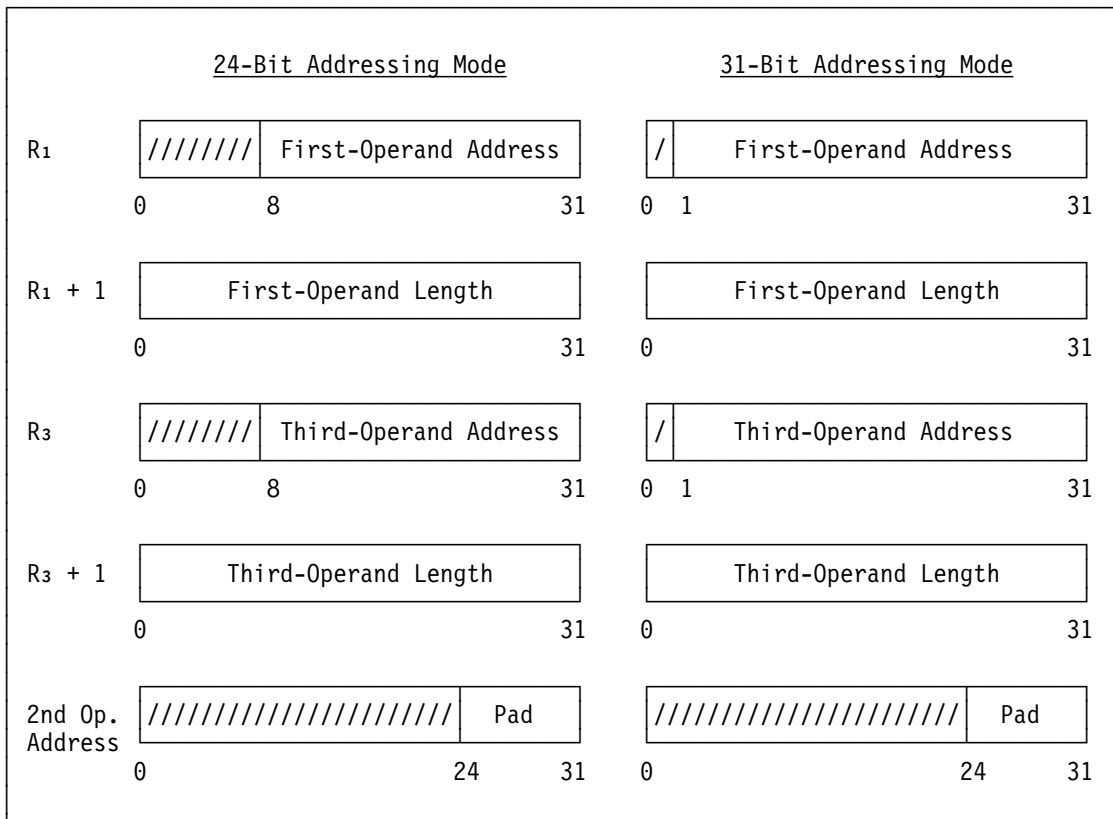
Figure 7-12. Register Contents and Second-Operand Address for MOVE LONG EXTENDED
