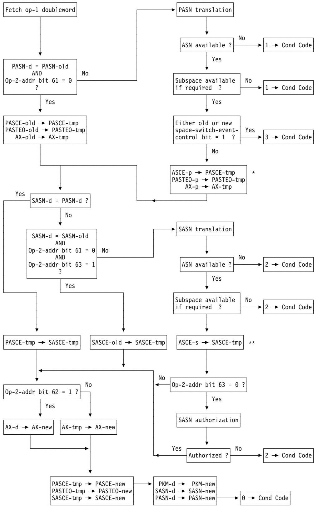
Figure 10-17. Execution of LOAD ADDRESS SPACE PARAMETERS
