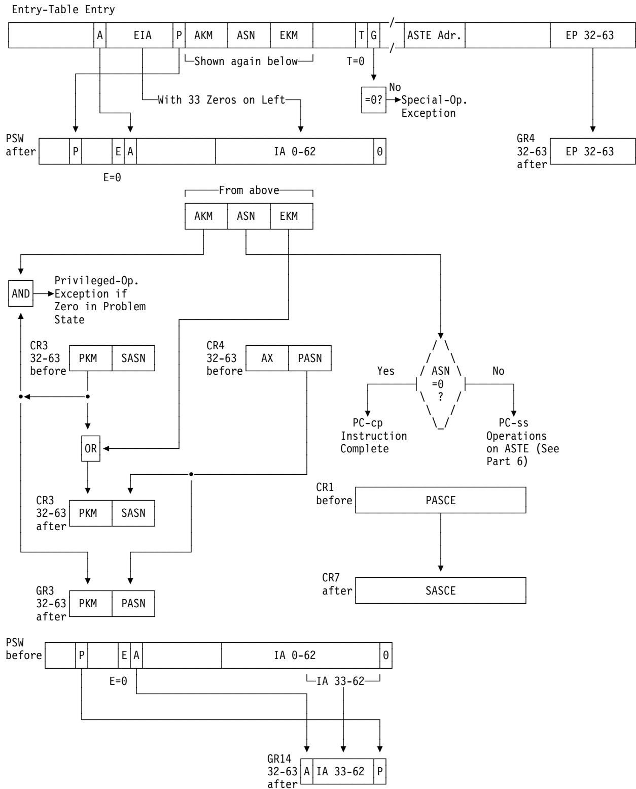
Figure 10-24 (Part 2 of 6). Execution of PROGRAM CALL
