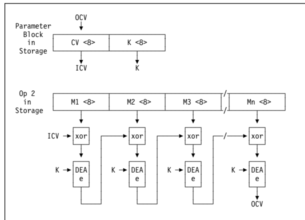
Figure 7-60. KMAC-DEA
