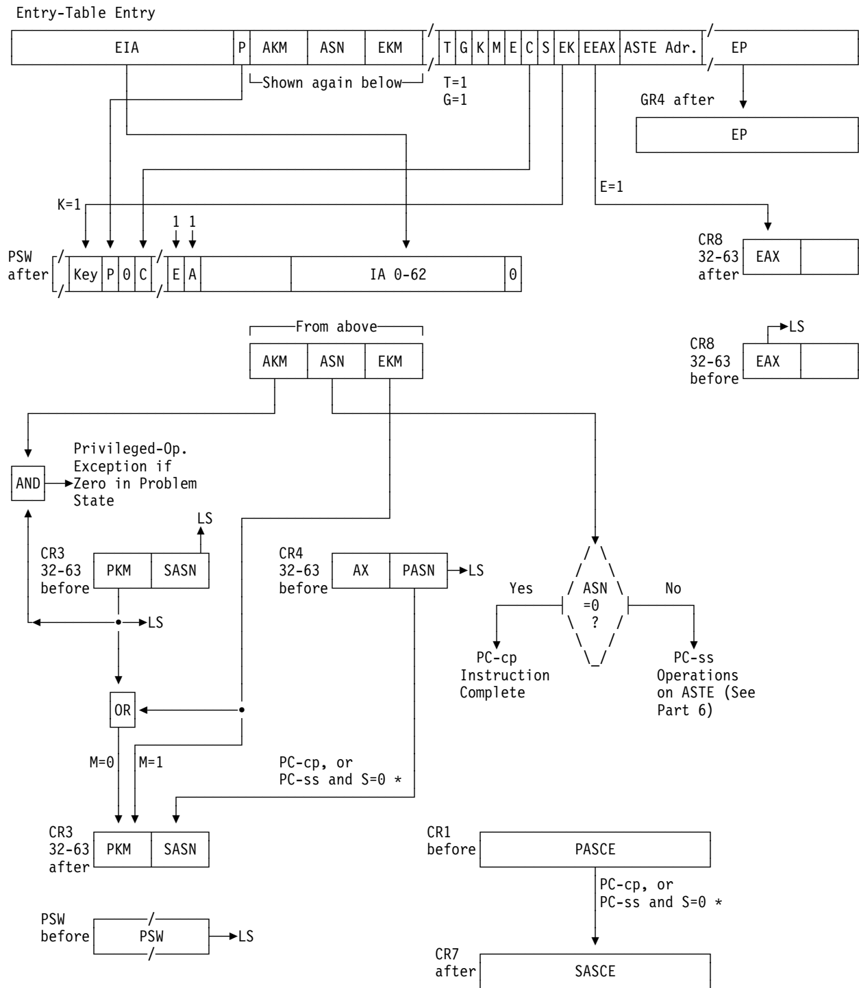
Figure 10-24 (Part 4 of 6). Execution of PROGRAM CALL
