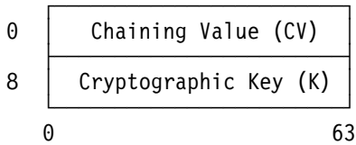
Figure 7-59. Parameter Block for KMAC-DEA
