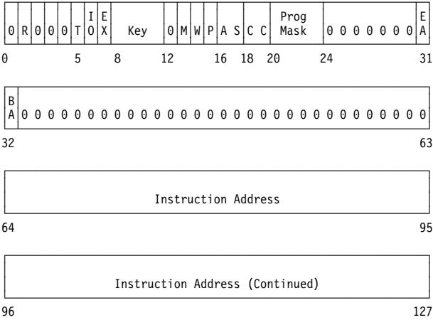
Figure 4-2. PSW Format
