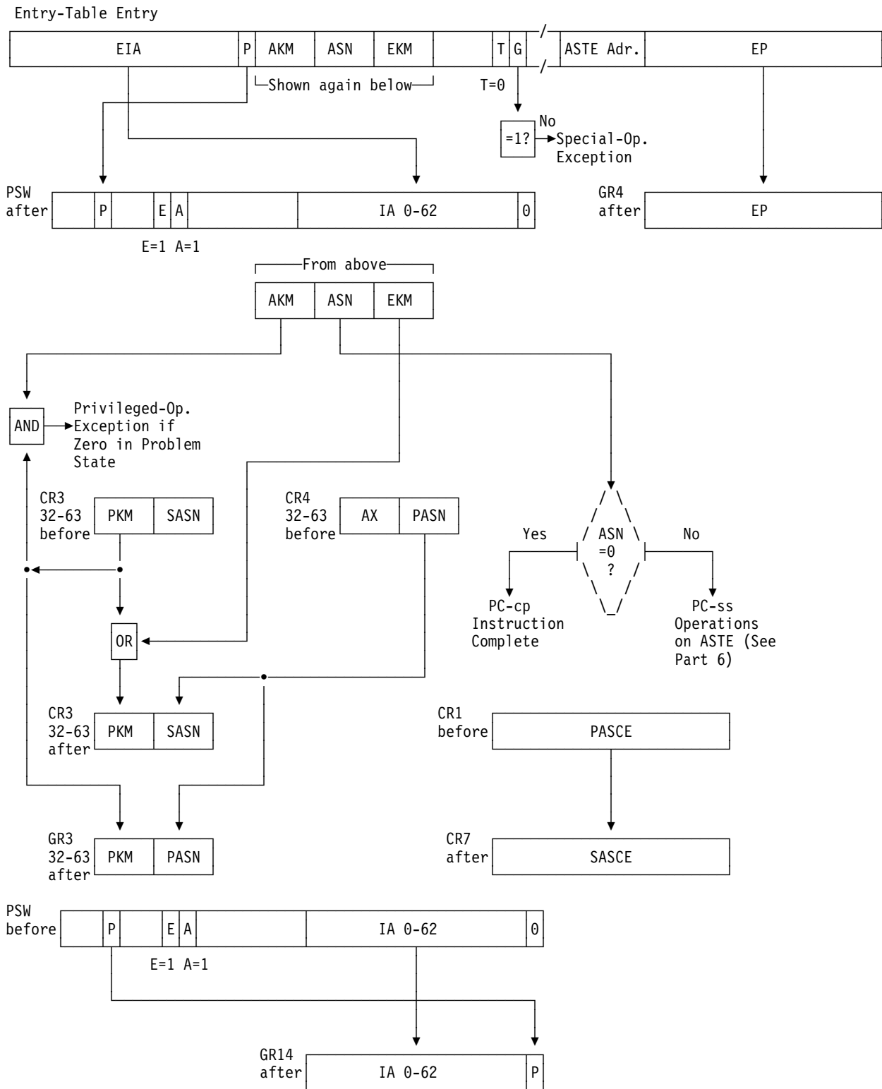
Figure 10-24 (Part 3 of 6). Execution of PROGRAM CALL
