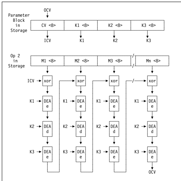
Figure 7-64. KMAC-TDEA-192
