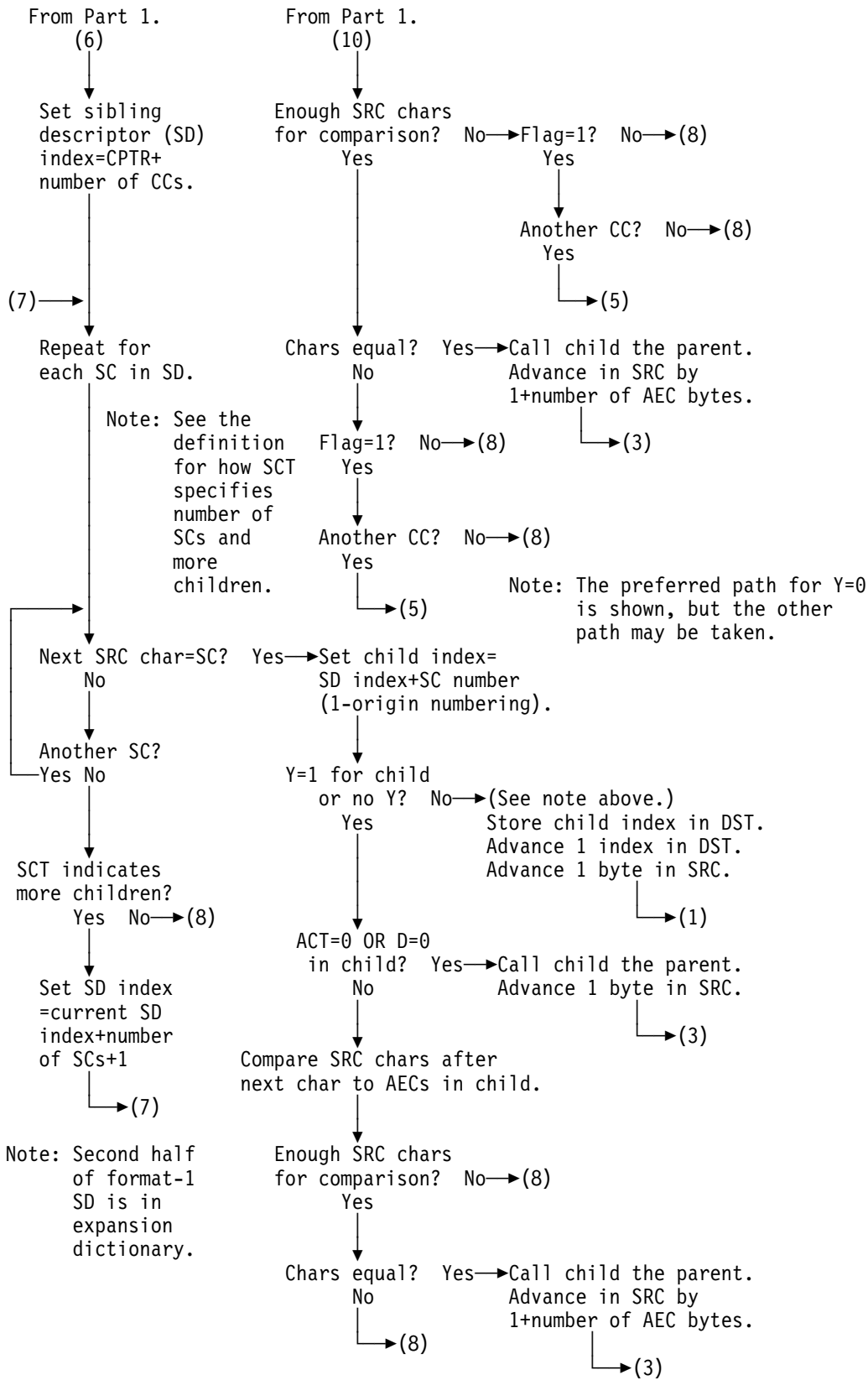
Figure 7-38 (Part 2 of 2). Compression Process
