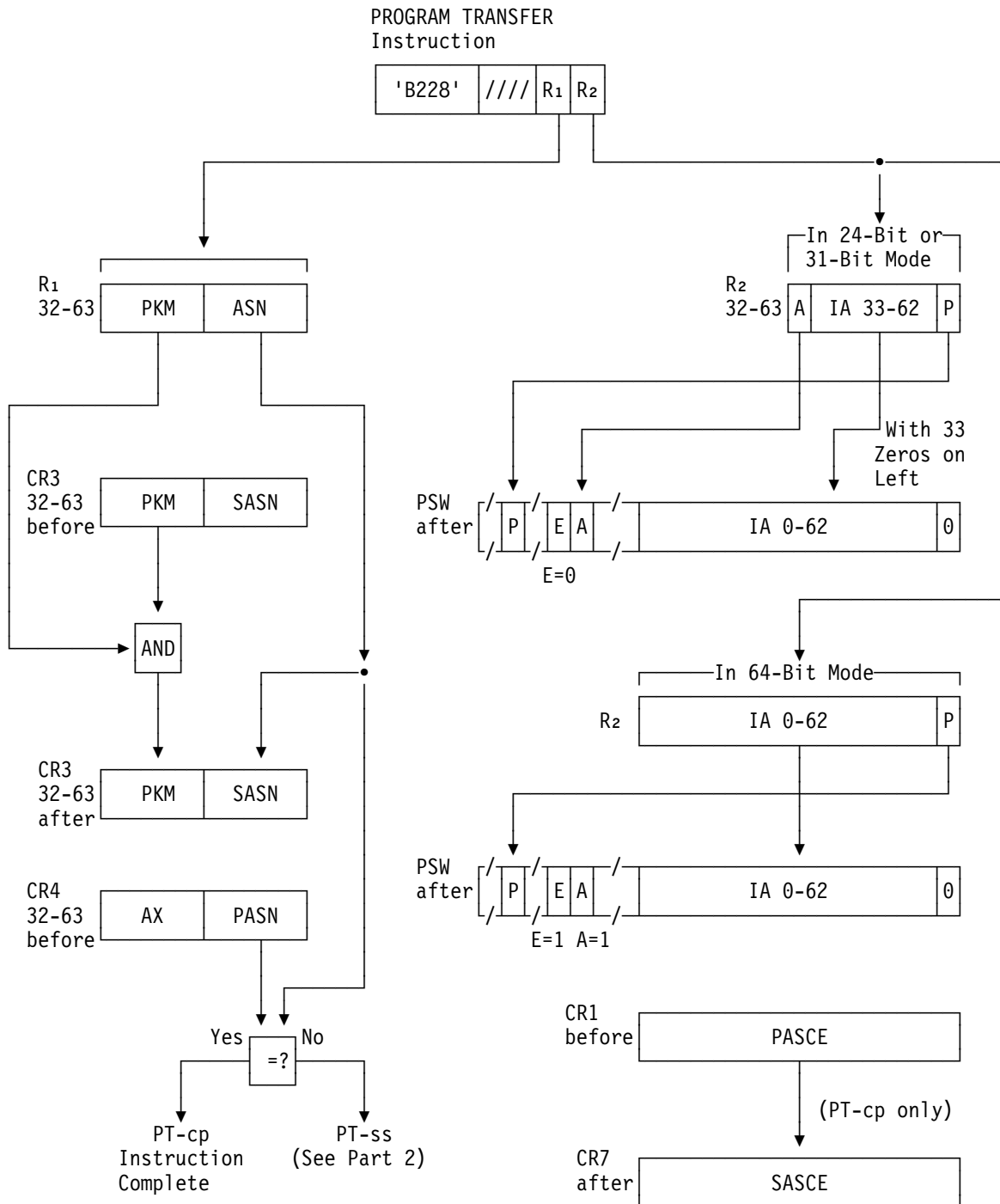
Figure 10-27 (Part 1 of 2). Execution of PROGRAM TRANSFER
