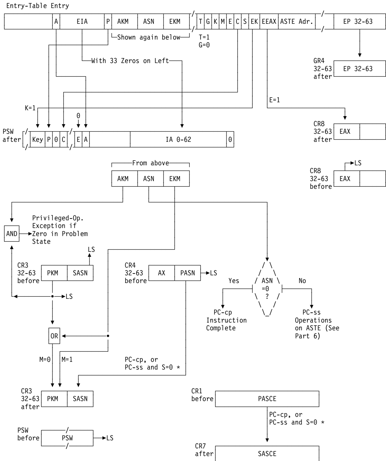
Figure 10-24 (Part 5 of 6). Execution of PROGRAM CALL
