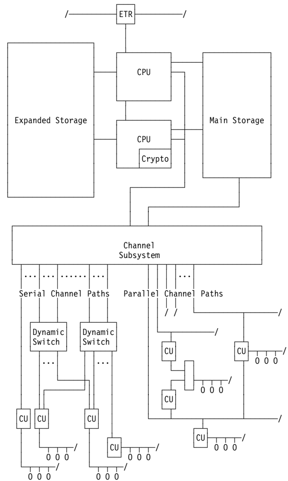
Figure 2-1. Logical Structure of a z/Architecture System with Two CPUs
