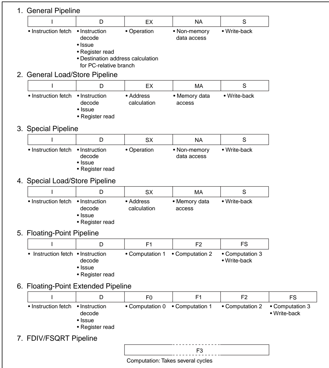
Figure 8.1 Basic Pipelines
