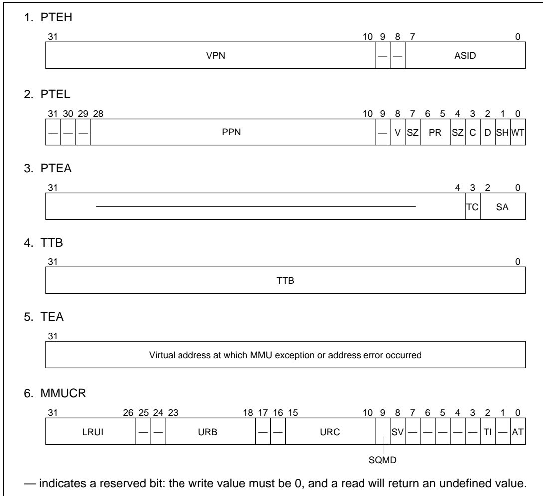
Figure 3.2 MMU-Related Registers
