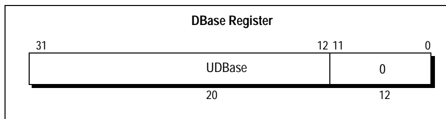
Figure 6.12 DBase Register
