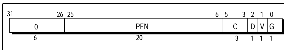
Figure 6.2 32-bit EntryLo0, EntryLo1 Register Fields in RC32364
