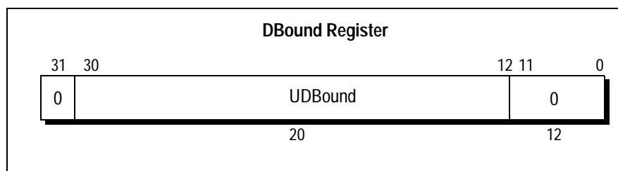
Figure 6.13 DBound Register
