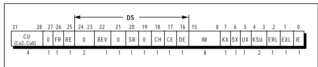
Figure 3.4 Status Register (4600/4700)
