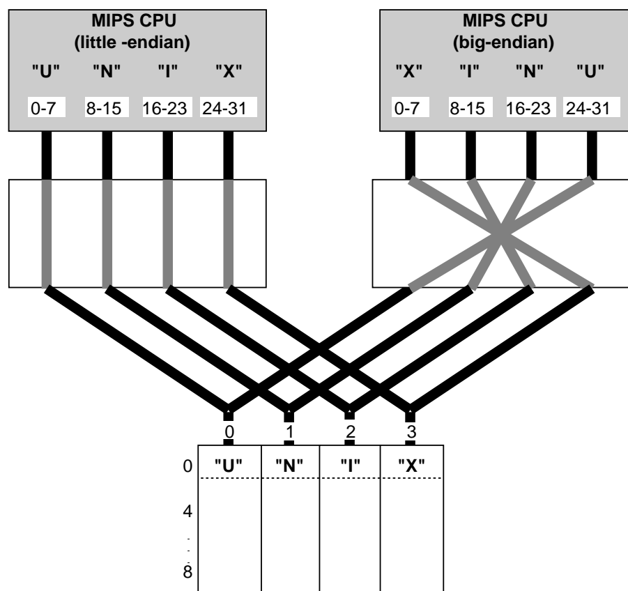
Figure 11.8 Byte-lane swapper
