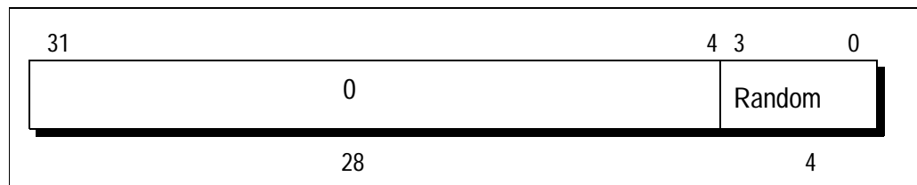
Figure 6.5 Random Register in RC32364
