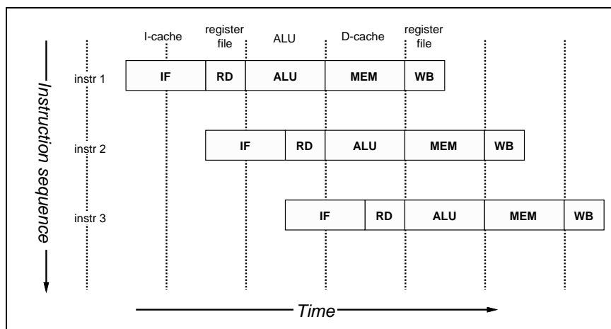
Figure 1.1 MIPS 5-stage pipeline
