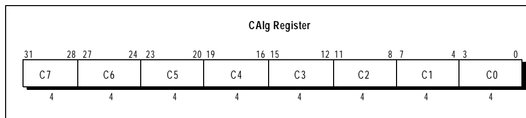
Figure 6.14 CAlg Register
