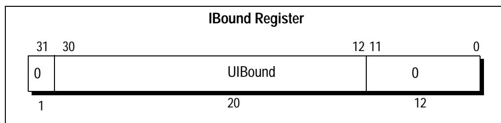
Figure 6.11 IBound Register
