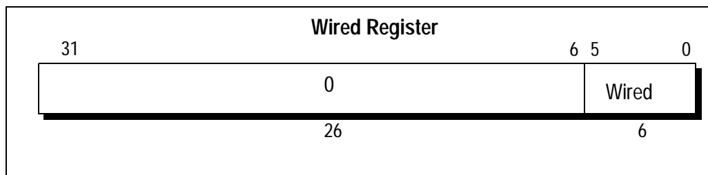
Figure 6.8 Wired Register
