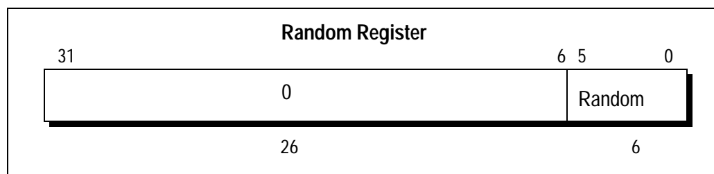
Figure 6.6 Random Register in RC4600/RC4700/RC5000
