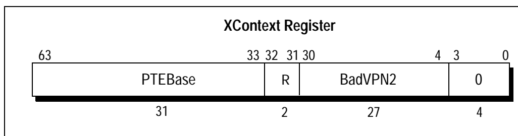
Figure 6.9 XContext Register Format
